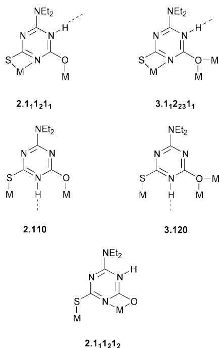
Scheme 3 Five possible bonding modes for OStaH − : the first four modes are displayed in compound 4. The numbers below each bonding mode refer to the Harris notation (see text). The fifth mode [2,1,1 2 ,1] is included to show how Harris notation distinguishes between possible binding modes ( cf. [2,1,1 2 ,1]). The dashed lines to H atoms indicate hydrogen bonds.
