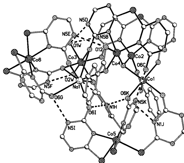
Fig. 6 The intra-molecular hydrogen bonding in compound 4 , shown as dashed lines. N...O contacts: N(5E)...O(12) 2.859, N(5F)...O(2W) 2.690, N(5I)...O(6G) 2.785, N(1J)...O(6K) 2.980, N(1H)...O(6K) 2.854, N(1H)...O(6I) 2.973, N(5K)...O(6C) 2.731, O(1W)...N(5D) 2.791, O(1W)...N(5B) 2.912, O(2W)...N(5H) 2.723 Å. Av. esd: 0.012 Å.
